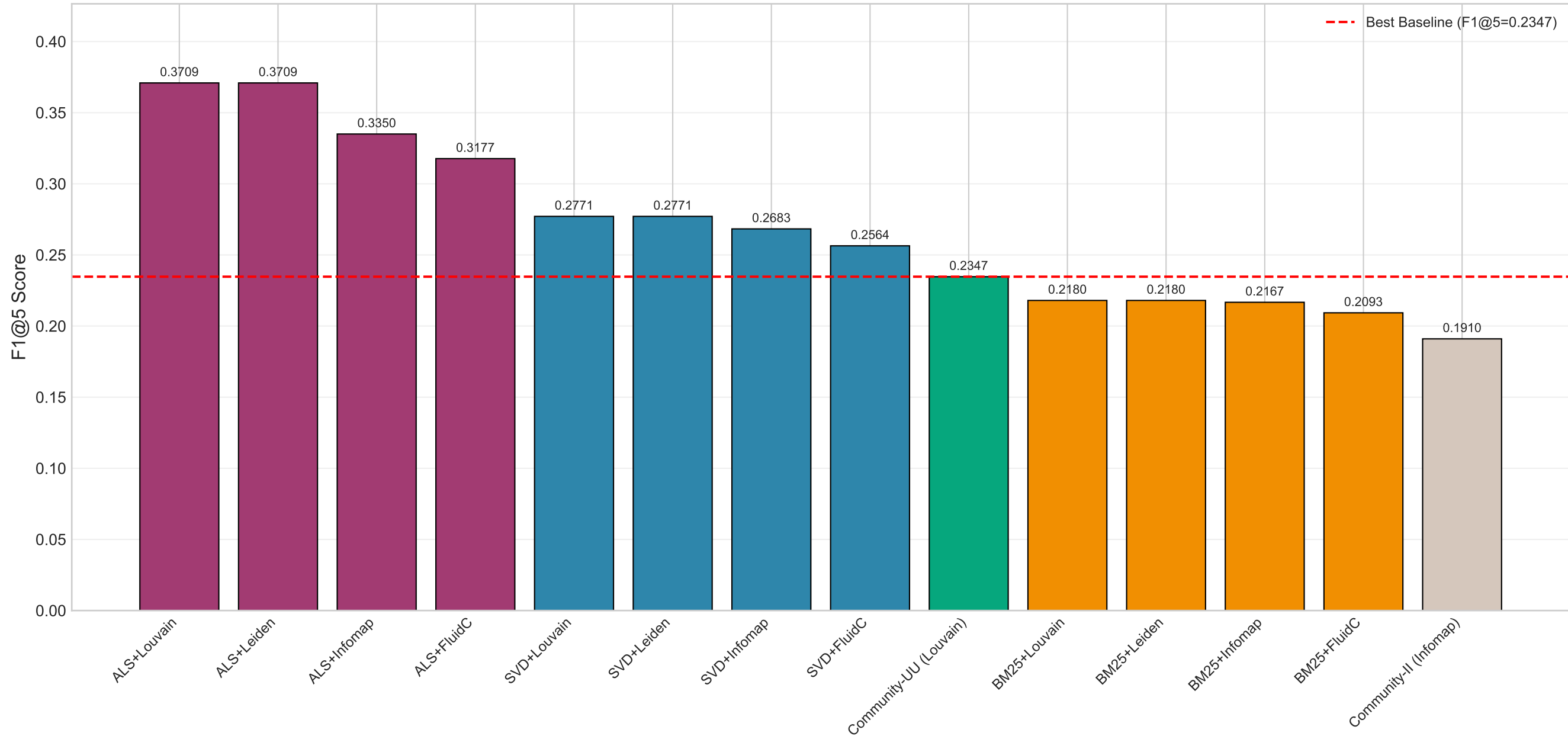
Figure 36: F1@5 Comparison of All Recommender Approaches
